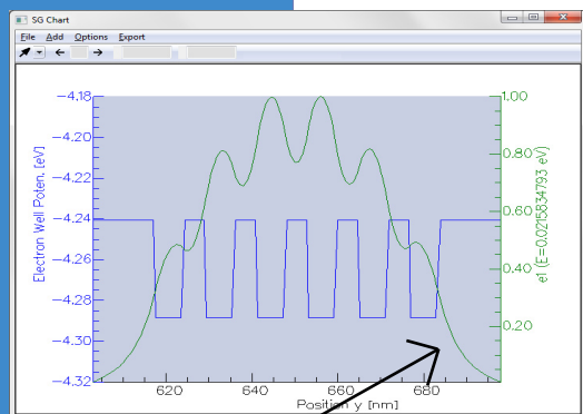
Carrier wavefunction
