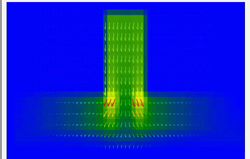
Current density plot showing current spreading in a ridge waveguide laser
