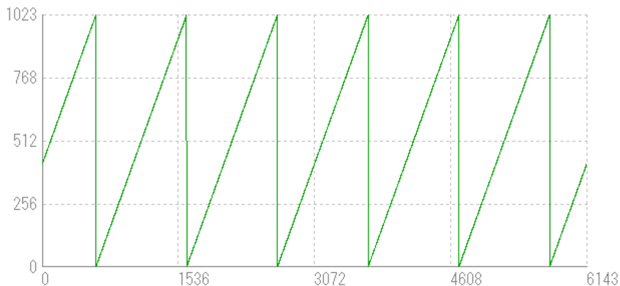
図 4-2-3-5 (C) RMSL6K17GE NED_GreyDiagonalRamp (10bit)
